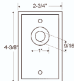
CM9080 Overall Dimension
