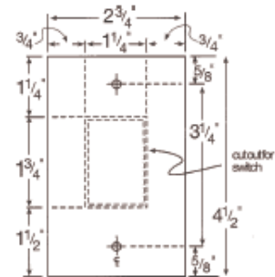
CM30 Cut Out
